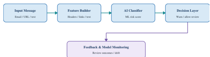
Figure 1. Proposed architecture of the AI-powered phishing detection system.
